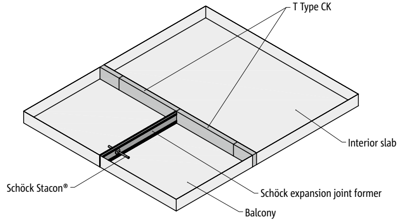
Fig. 28: Schöck Isokorb® Type CK: The expansion joint former
