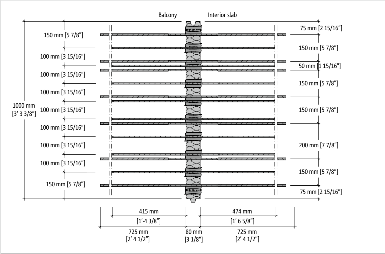
Fig. 16: Schöck Isokorb® T Type CK-M6-V3: Top view of the product
