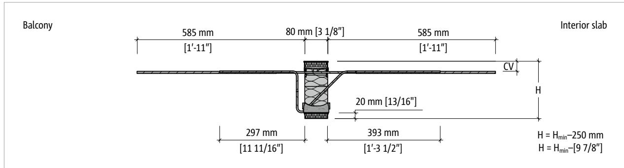
Fig. 7: Schöck Isokorb® T Type CK-M1-V1 to M6-V1: Product cross-section
