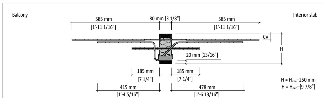
Fig. 12: Schöck Isokorb® T Type CK-S-M6-V2: Product cross-section
