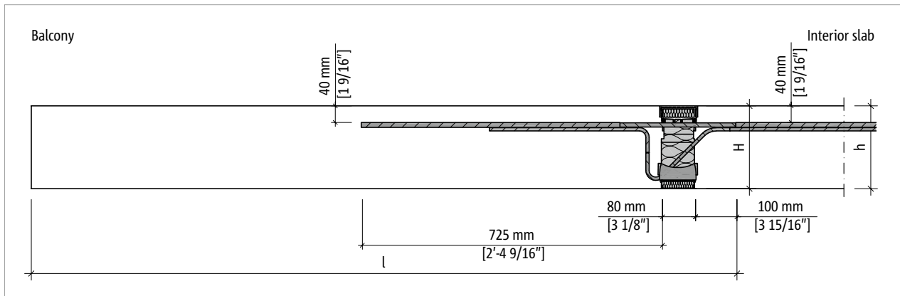
Fig. 5: Schöck Isokorb® T Type CK: Concrete cover CV40 [1.5"] with flat balcony slab
