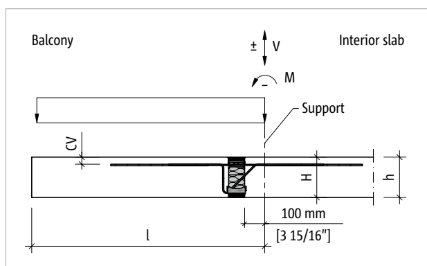
Fig. 19: Schöck Isokorb® T Type CK: Structural system
