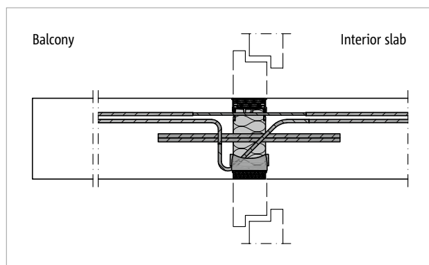
Fig. 3: Schöck Isokorb® T Type CK-S: Balcony with window wall system
