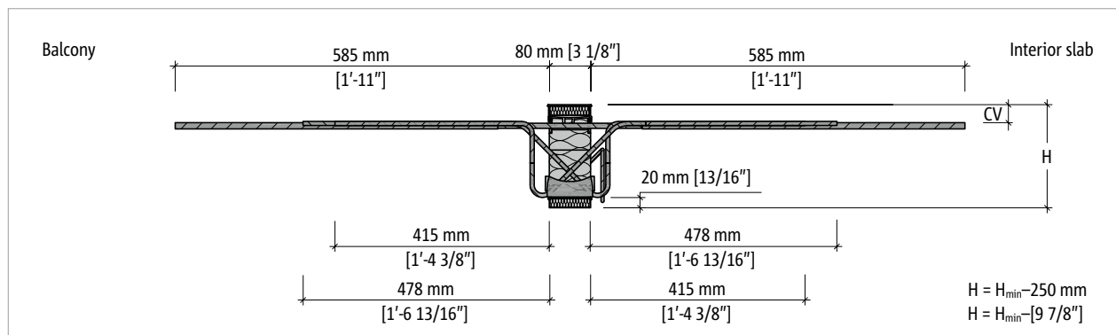
Fig. 11: Schöck Isokorb® T Type CK-M6-VV1 to M11-VV1: Product cross-section
