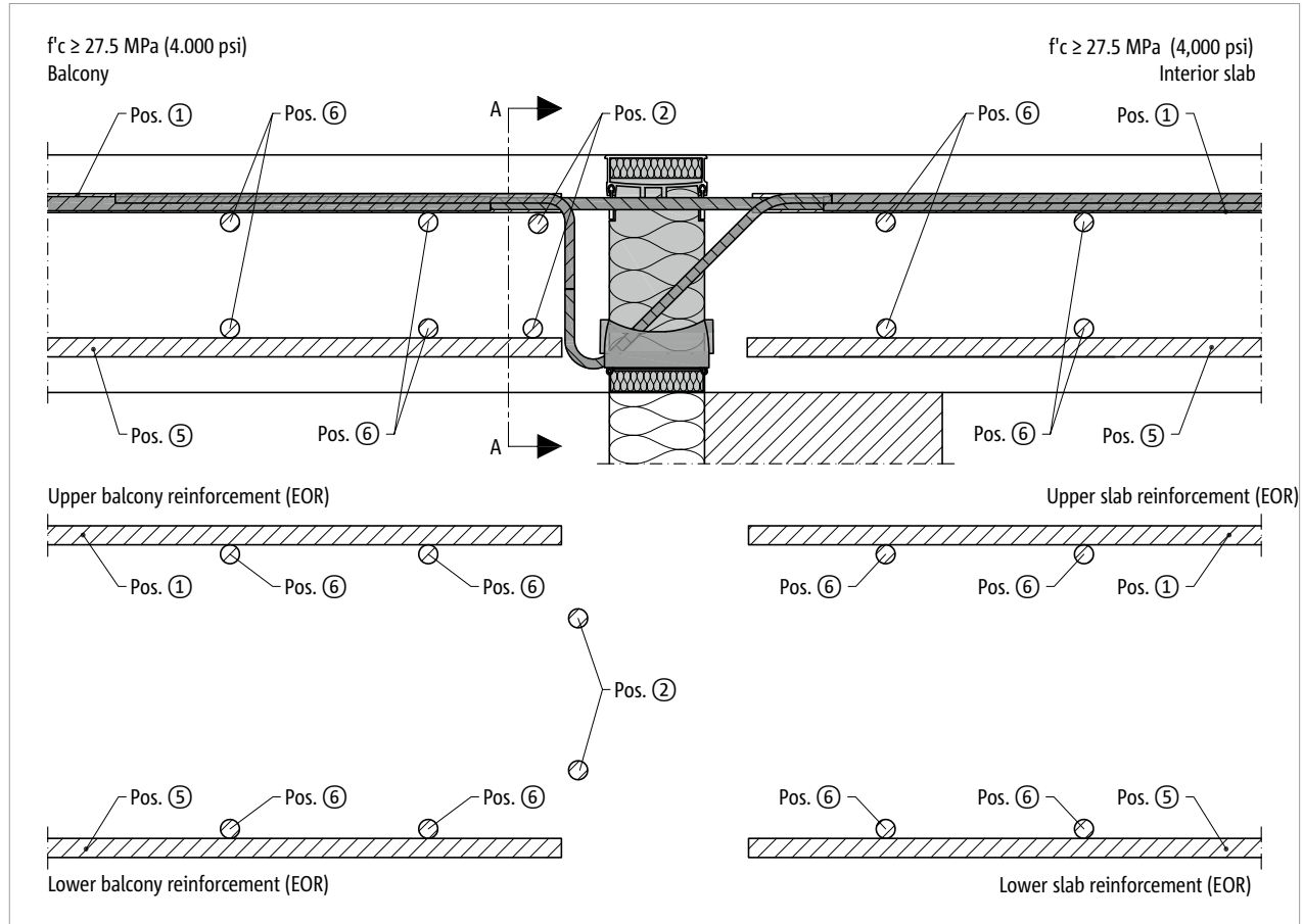
Fig. 21: Schöck Isokorb® T Type CK: Cross section of recommended cast-in-place reinforcement (supplied by others) - direct support
