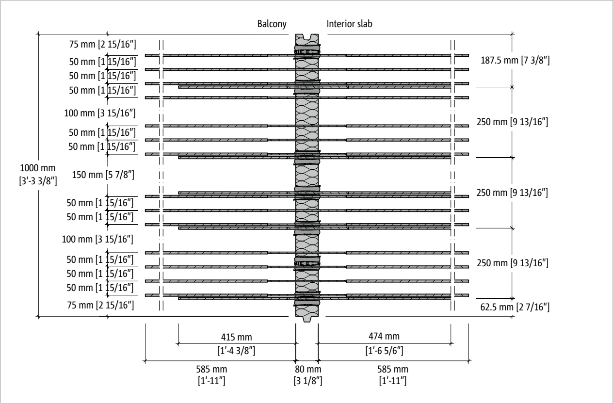
Fig. 15: Schöck Isokorb® T Type CK-M5-V2: Top view of the product
