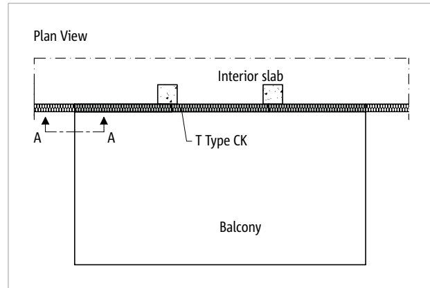
Fig. 23: Schöck Isokorb® T Type CK: Location of section A-A
