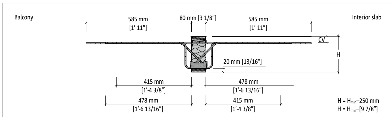
Fig. 10: Schöck Isokorb® T Type CK-M4-VV1 to M5-VV1: Product cross-section
