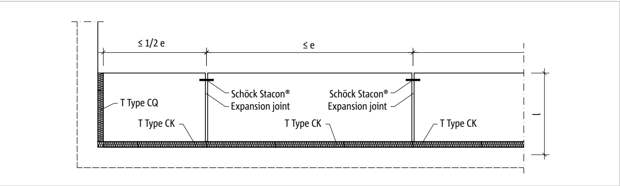
Fig. 27: Schöck Isokorb® Type CK: Maximum expansion joint spacing
