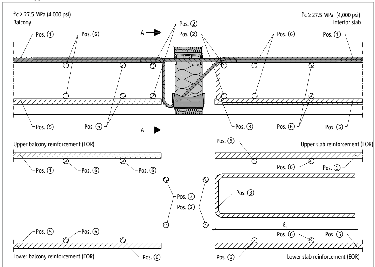
Fig. 24: Schöck Isokorb® T Type CK: Cross section of recommended cast-in-place reinforcement (supplied by others) - indirect support
