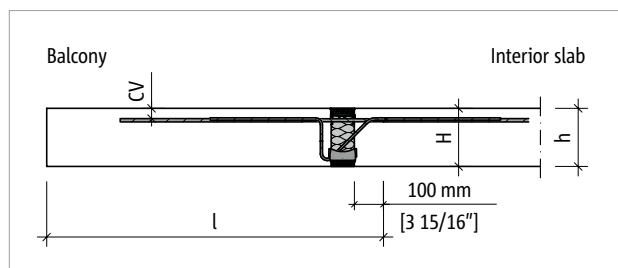
Fig. 25: Schöck Isokorb® T Type CK: Structural system
