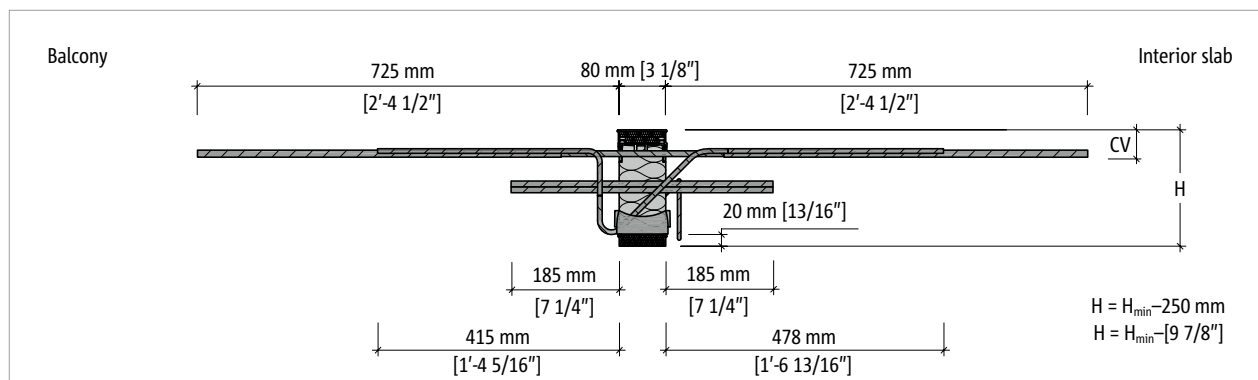
Fig. 13: Schöck Isokorb® T Type CK-S-M8-V1 and M11-V1: Product cross-section
