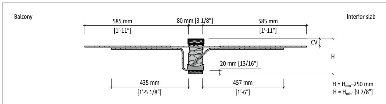
Fig. 8: Schöck Isokorb® T Type CK-M1-V2 to M6-V2: Product cross-section
