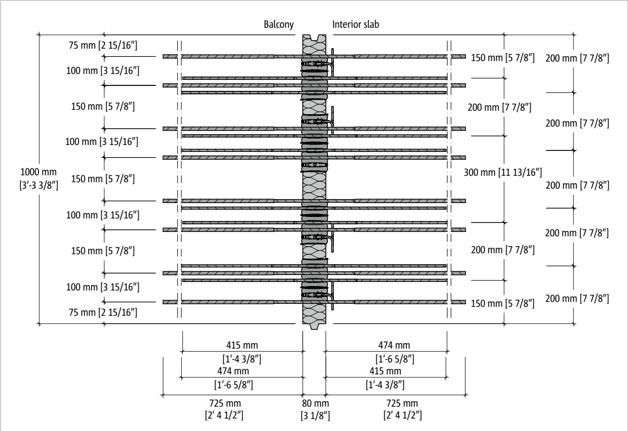
Fig. 17: Schöck Isokorb® T Type CK-M6-VV1: Top view of the product
