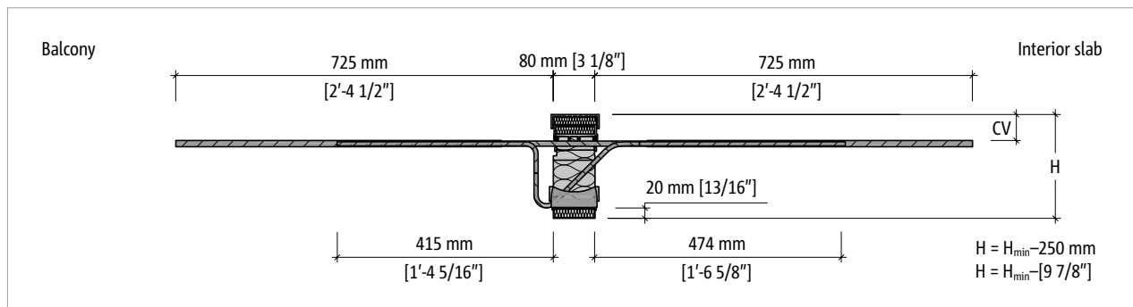
Fig. 9: Schöck Isokorb® T Type CK-M6-V3 to M11-V1: Product cross-section
