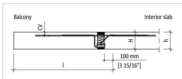
Fig. 26: Schöck Isokorb® T Type CK: Structural system
