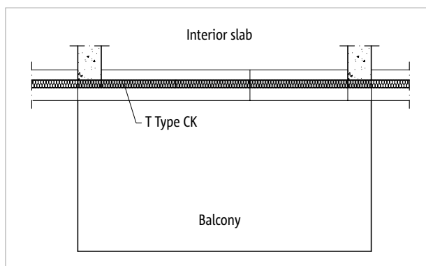
Fig. 4: Schöck Isokorb® T Type CK: Cantilever balcony
