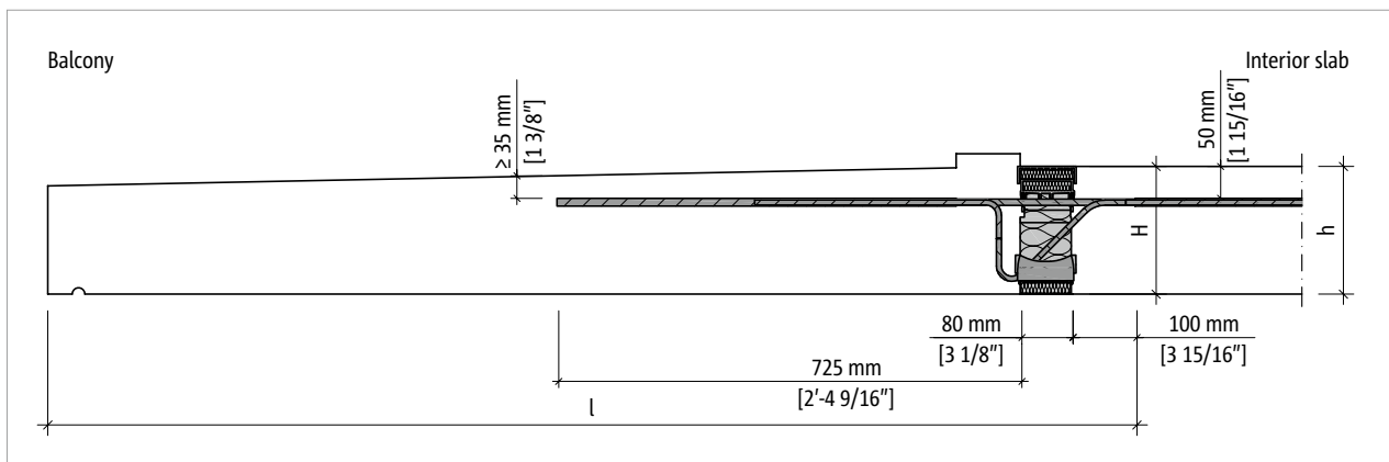
Fig. 6: Schöck Isokorb® T Type CK: Concrete cover CV50 [2"] with sloped balcony slab
