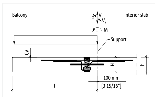
Fig. 20: Schöck Isokorb® T Type CK-S: Structural system
