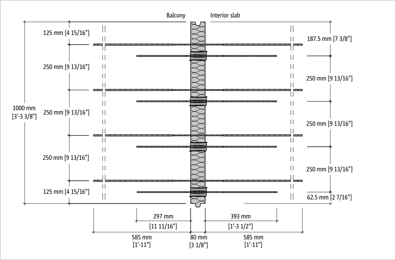
Fig. 14: Schöck Isokorb® T Type CK-M1-V1: Top view of the product
