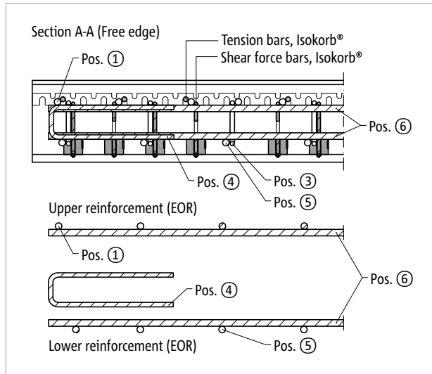
Fig. 22: Schöck Isokorb® T Type CK: Section A-A Depiction of free balcony edge
