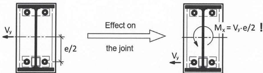
Figure 3: Torsional moment from misalignment of the shear force transfer (example using configuration 'S-2')
