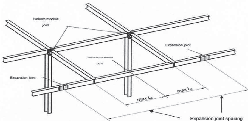
Figure 4: Maximum influence length
