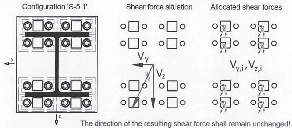
Figure 2: Principle of shear force allocation to the S-V modules of a joint
