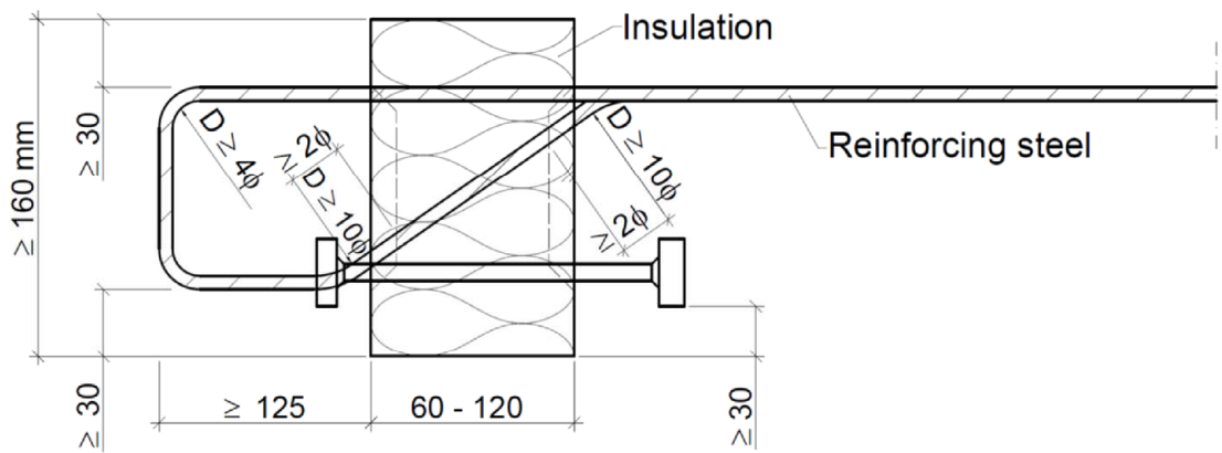
Fig. 18: Schöck Isokorb® type O with SCE
