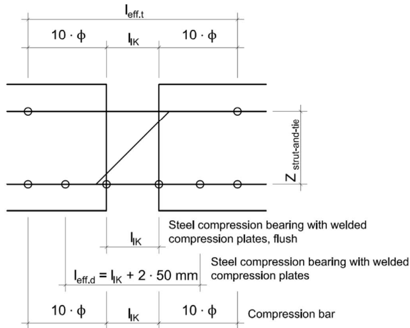
Fig. 50: l_{eff} for ribbed stainless steel bar, as per section A.3
