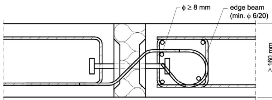
Fig. 48: Example of a Schöck Isokorb® type Q type Q with SCE and execution as edge beam
