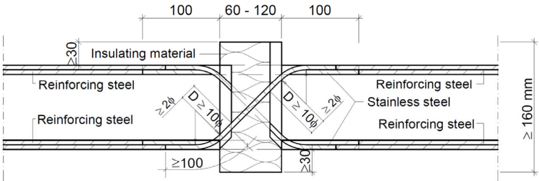
Fig. 23: Schöck Isokorb® type D with SCE
