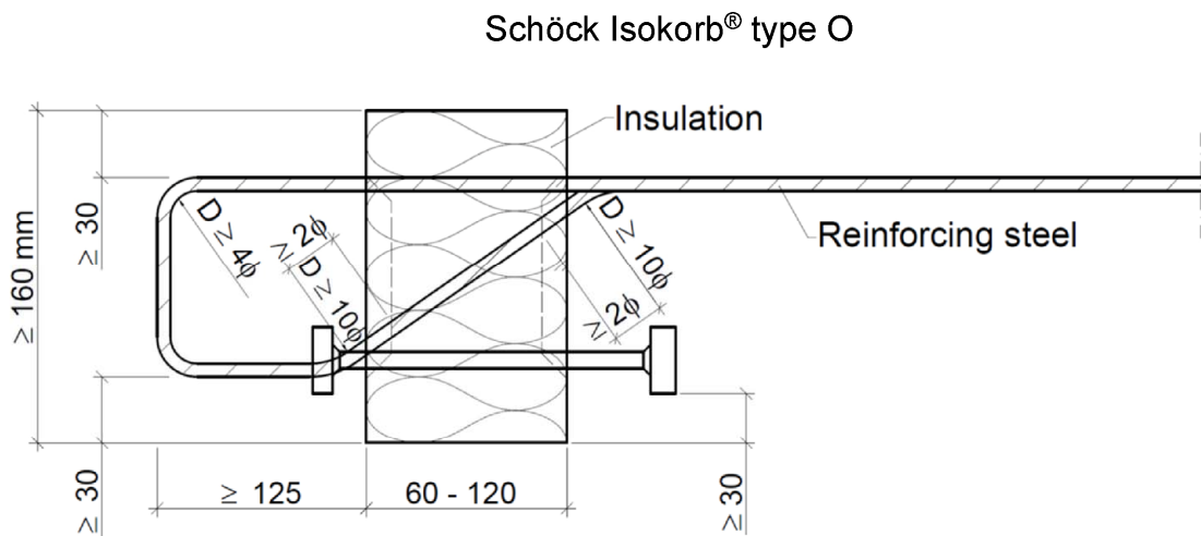
Fig. 18: Schöck Isokorb® type O with SCE
