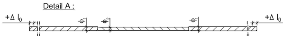
Fig. 12: tension bar (type K) with diameter combination
