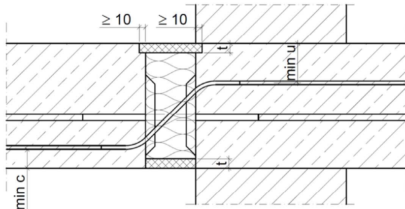
Fig. 34: Schöck Isokorb® type Q with SCE
