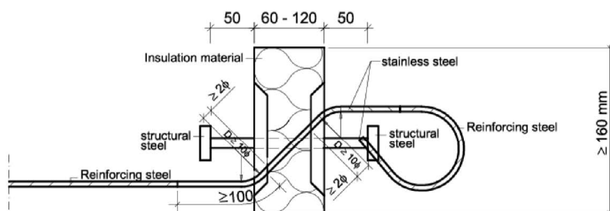
Fig. 47: Schöck Isokorb® type Q with SCE
