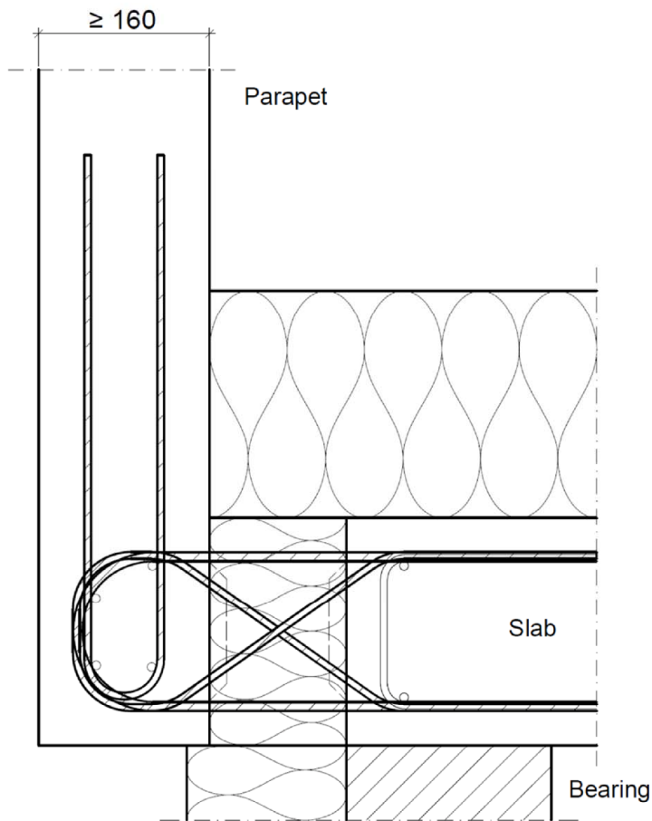
Fig. 28: Example of a Schöck Isokorb® type F with SCE with on-site reinforcement
