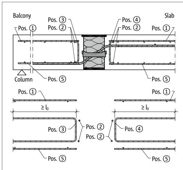
Fig. 132: Schöck Isokorb® XT type Q-V5 to Q-V11: On-site reinforcement
