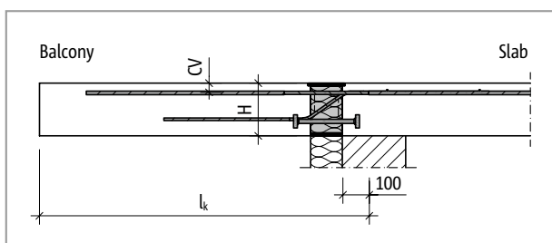
Fig. 32: Schöck Isokorb® XT type K-M11: Static system
