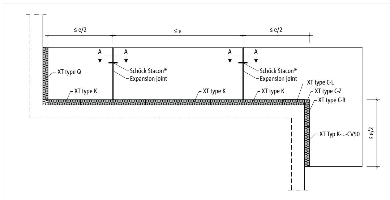
Fig. 17: Schöck Isokorb® XT type K: Expansion joint formation with longitudinally displaceable shear force dowel, e.g. Schöck Stacon®
