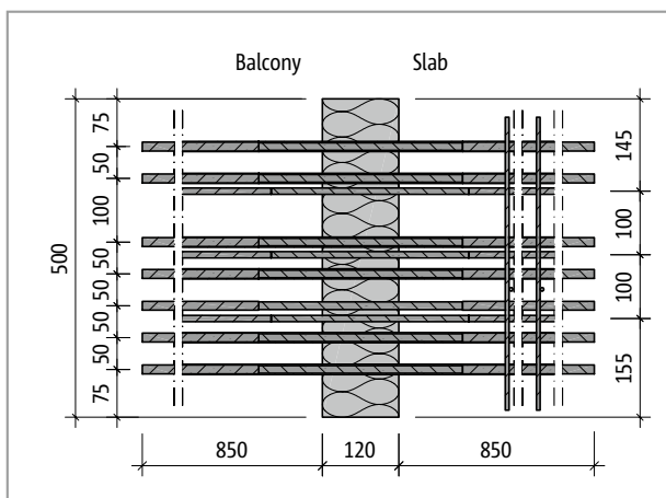
Fig. 43: Schöck Isokorb® XT type K-M12: Product layout
