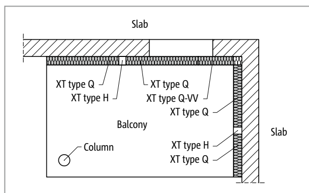
Fig. 214: Schöck Isokorb® XT type H: Balcony supported on two sides using columns
