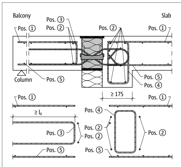
Fig. 133: Schöck Isokorb® XT type Q-VV1 to VV4 on-site reinforcement in downstand beam
