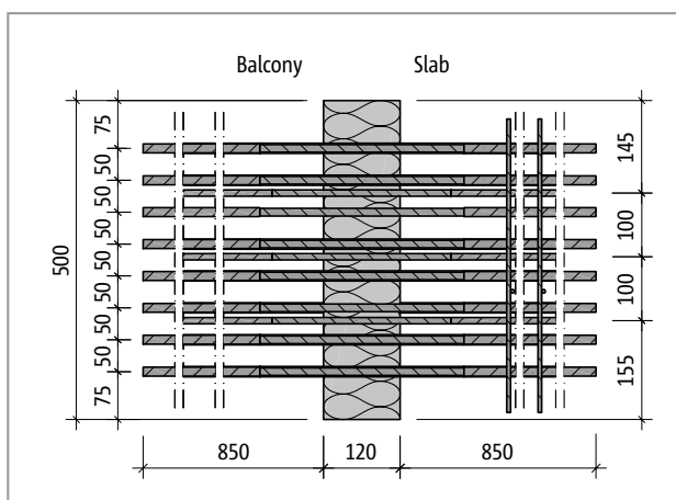
Fig. 44: Schöck Isokorb® XT type K-M13: Product layout
