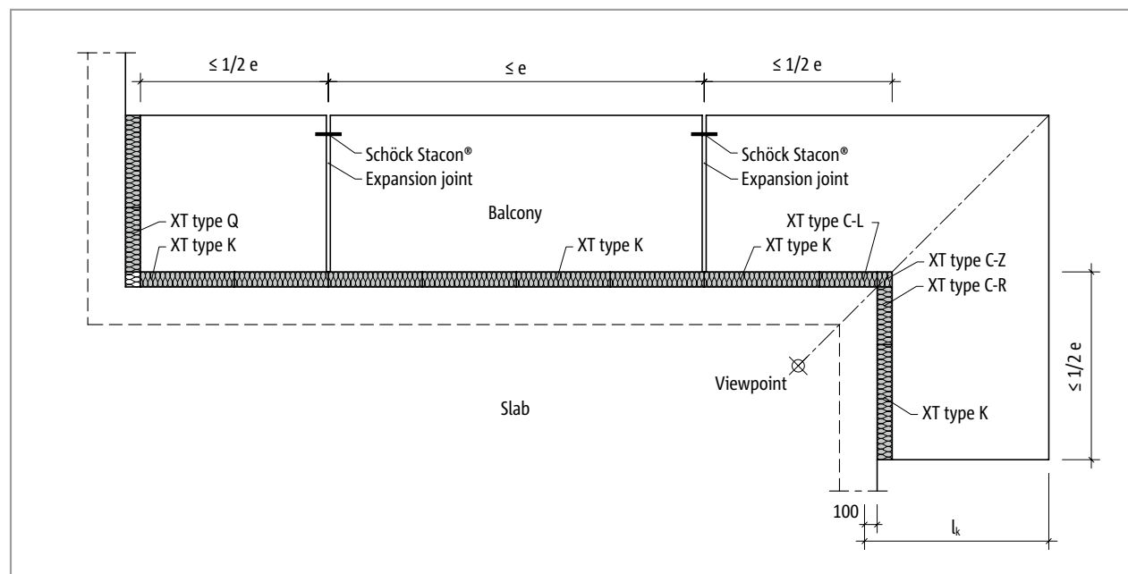
Fig. 196: Schöck Isokorb® XT type C: Expansion joint arrangement
