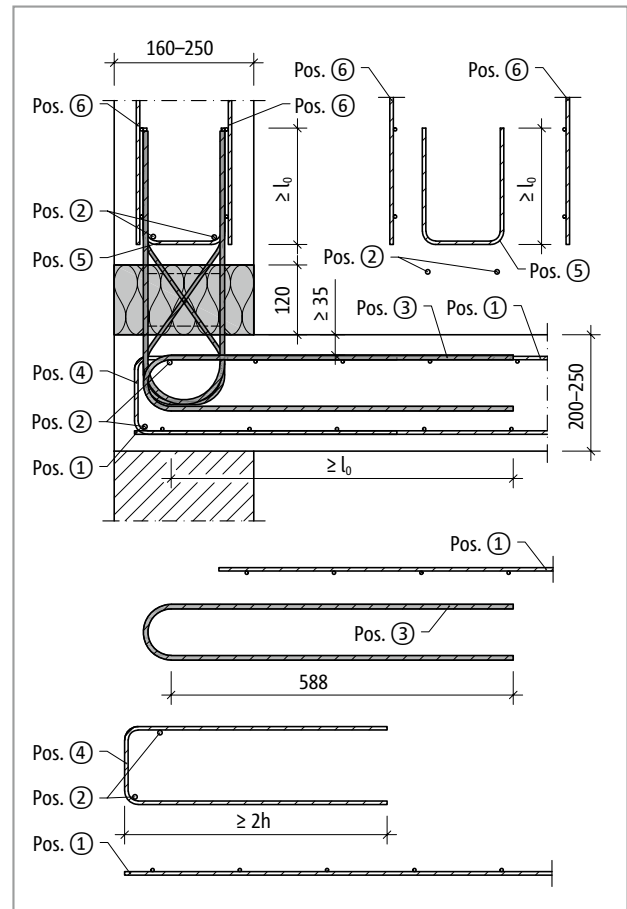
Fig. 269: Schöck Isokorb® XT type A: On-site reinforcement outside
