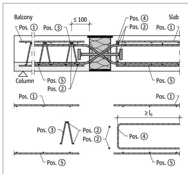
Fig. 173: Schöck Isokorb® XT type Q-P-VV: On-site reinforcement, balcony side with lattice beam
