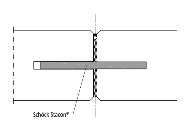
Fig. 18: Schöck Stacon®: Expansion joint formation in in-situ concrete
