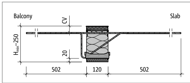
Fig. 34: Schöck Isokorb® XT type K-M1 to M4: Product section
