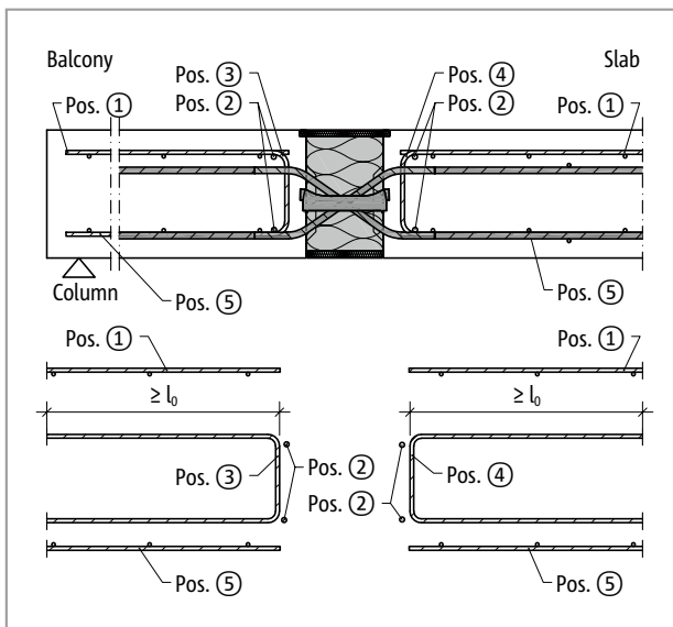
Fig. 134: Schöck Isokorb® XT type Q-VV5 to VV11 on-site reinforcement
