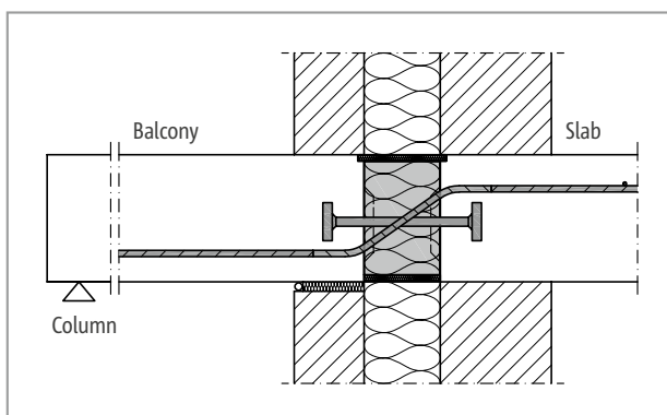
Fig. 148: Schöck Isokorb® XT type Q-P: Connection supported balcony with thermal insulating cavity masonry
