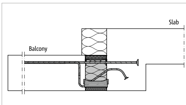
Fig. 4: Schöck Isokorb® XT type K-U...-REI120: Fire protection board top and bottom; lateral integrated fire protection bands
