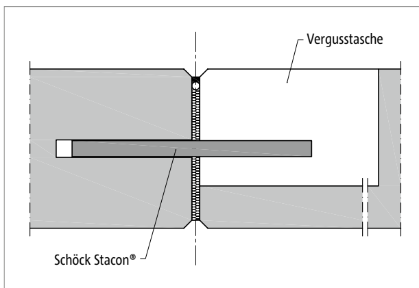
Fig. 19: Schöck Stacon®: Expansion joint formation precast concrete balcony
