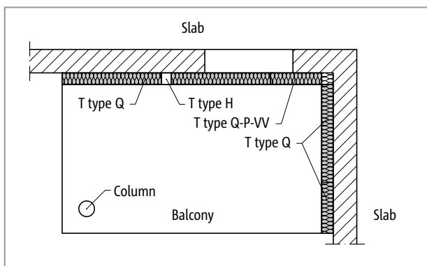
Fig. 143: Schöck Isokorb® XT type Q, Q-P-VV: Balcony supported on two sides with column and positive shear forces
