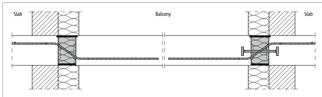
Fig. 146: Schöck Isokorb® XT type Q-P, Q-Z: Application case recessed balcony see page 116
