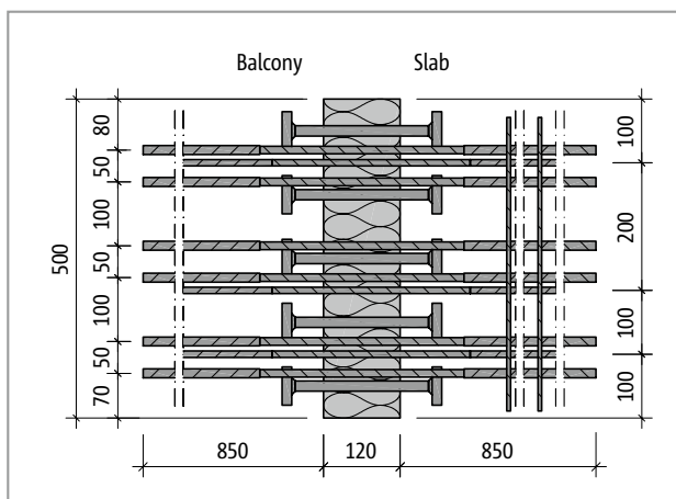
Fig. 42: Schöck Isokorb® XT type K-M11: Product layout
