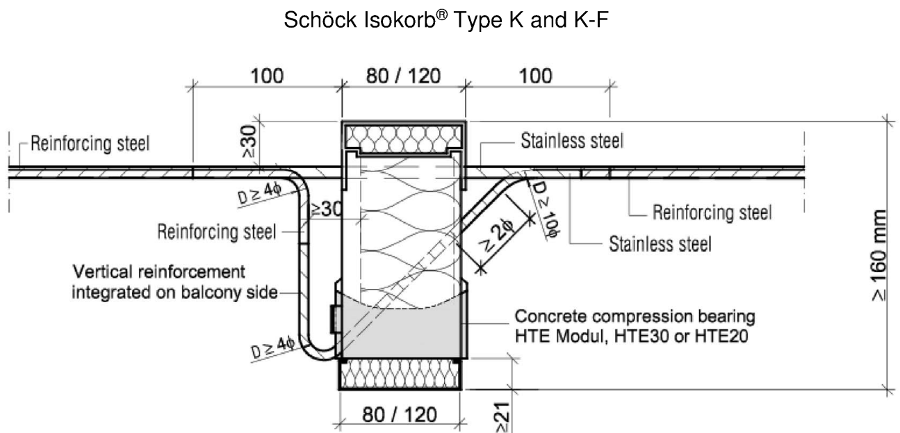
Fig. 17: Schöck Isokorb® type K with CCE
